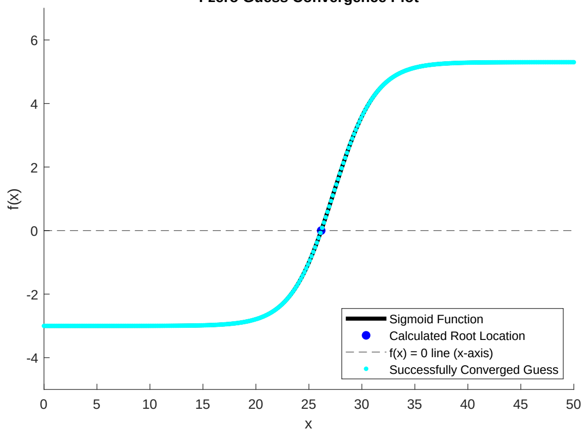
Fzero Guess Convergence Plot
